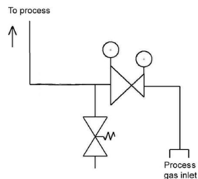
FLOW DIAGRAM
