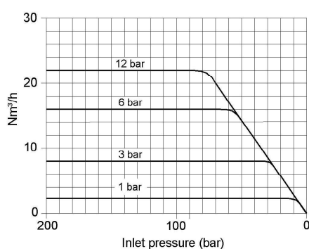
PERFORMANCE CURVE
