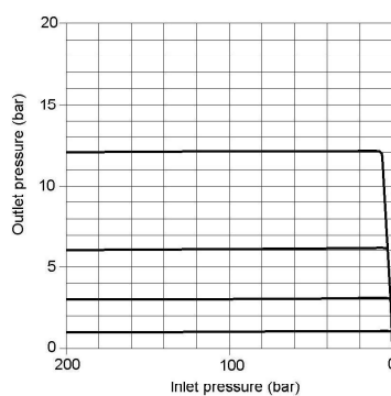
DYNAMIC FLOW CURVE
